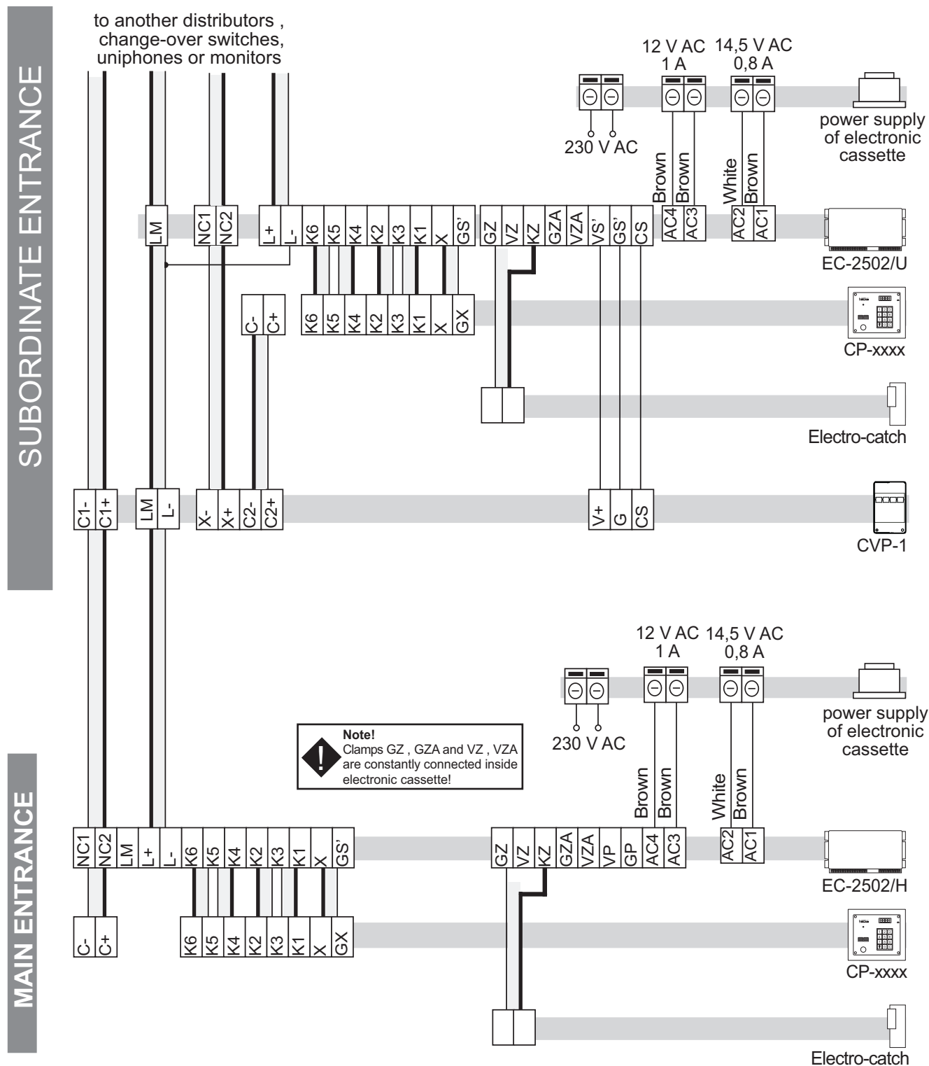
Figure 7: Connecting outer panel to system CD-2502 in video version – multi-entry system
