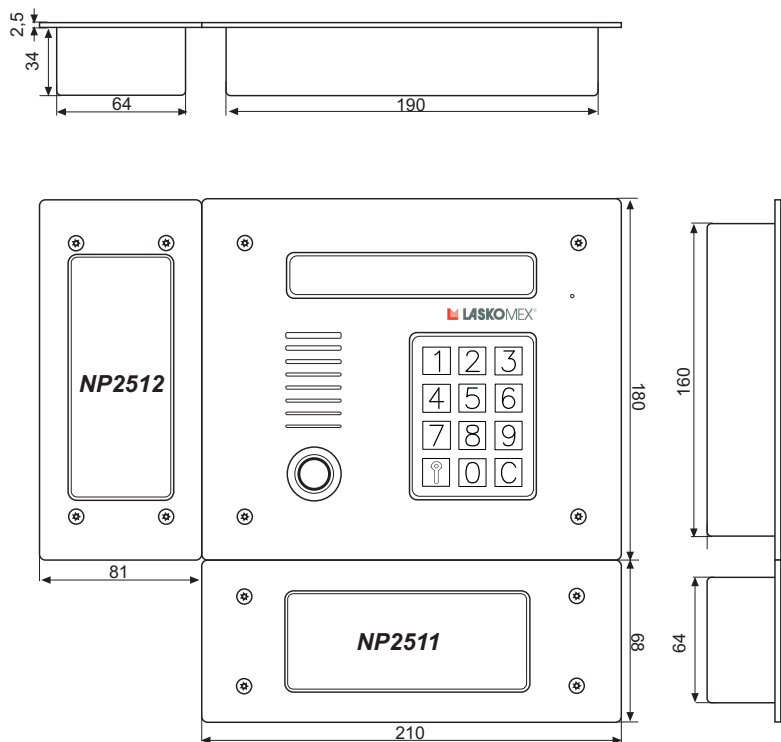
Figure 11: Dimensions of panels CP-2510 and CP-2513, NP2512 and NP2511
