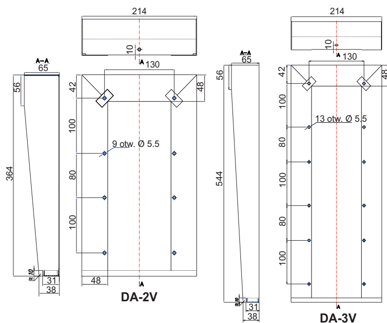
Figure 9: Dimensions of over-plaster casing in vertical position for CP-2502xx and CP-2503xx panels
