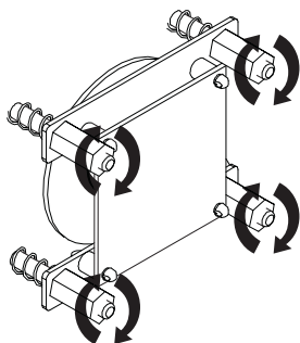
Figure 5: The way of adjustment of camera position in the external panel in video version - not applicable to CP-2502
