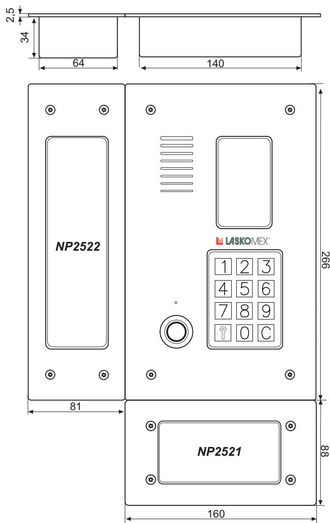
Figure 14: Dimensions of panels CP-2520, CP-2523, NP2522 and NP2521
