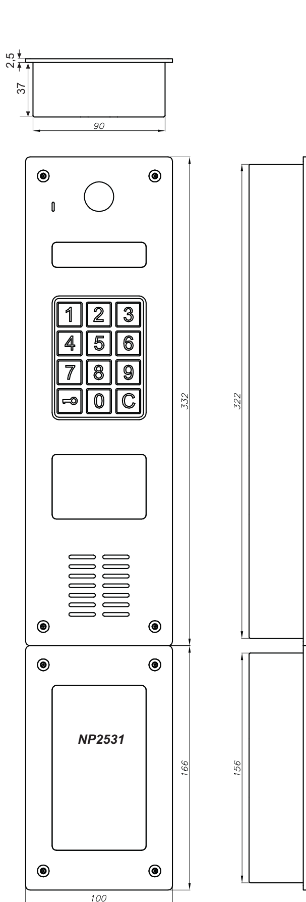
Figure 17: Dimensions of panels CP-2530, CP-2533
