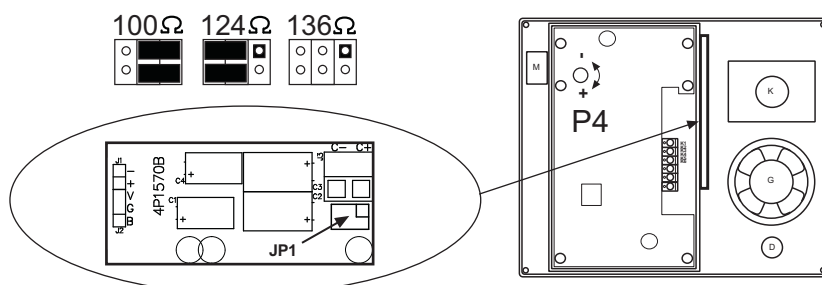
Figure 4: External panel - setting output impedance in a panel in video version - not applicable for CP-2530 and CP-25x3 panels.
