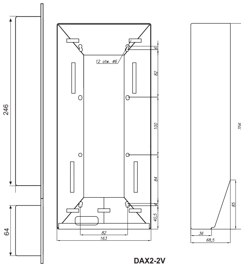
Figure 15: Dimensions of over-plaster casing in vertical position for CP-2520 and CP-2523 panels
