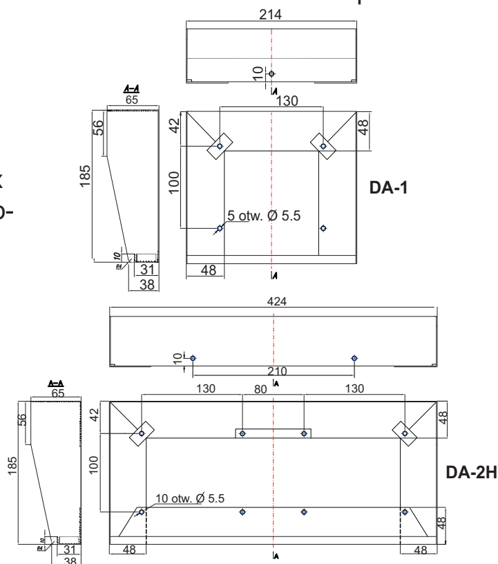
Figure 9: Dimensions of over-plaster casing in vertical position for CP-2502xx and CP-2503xx panels
