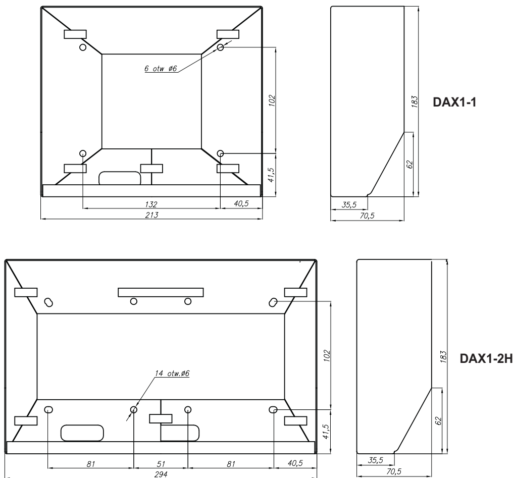
Figure 12: Dimensions of over-plaster casing in vertical position for CP-2510 and CP-2513 panels
