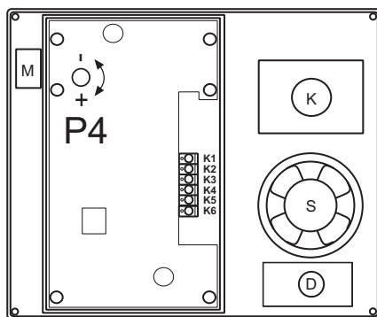
Figure 2: Position of the potentiometer P4 in the external panel - in CP-2502.
