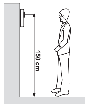
Figure 6: Recommended height of panel mounting.
