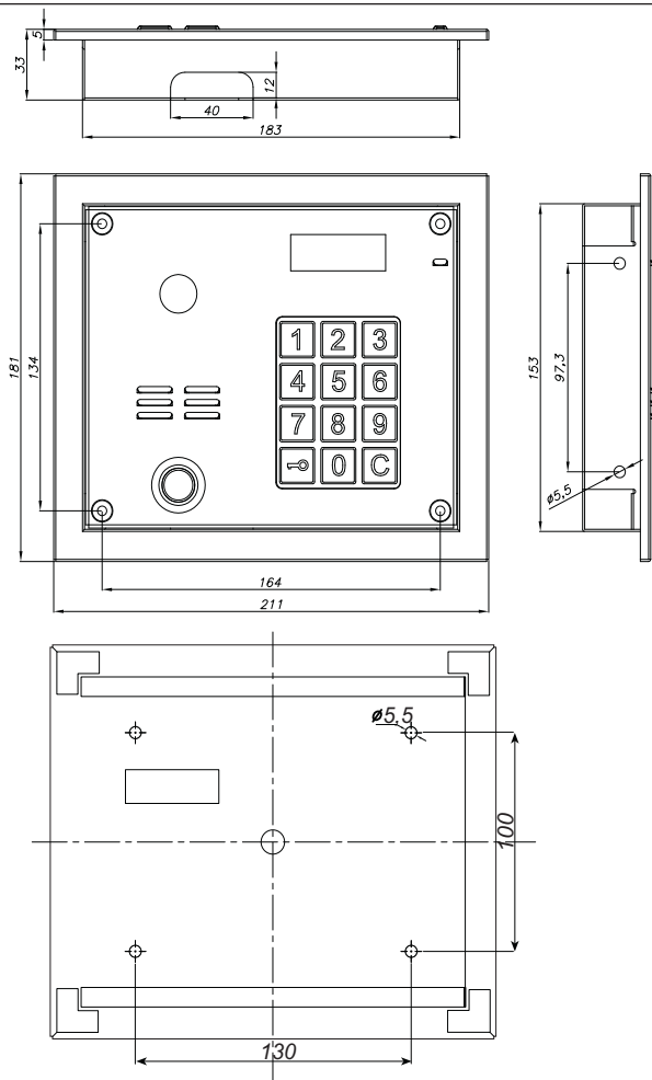
Figure 8: Dimensions of panels CP-2502xx and CP-2503xx with the frame for sub-plaster assembly
