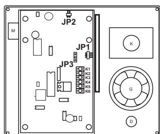
Figure 3: External panel - setting the kind of used display and supplying camera (only in video version) - in CP-2503.
