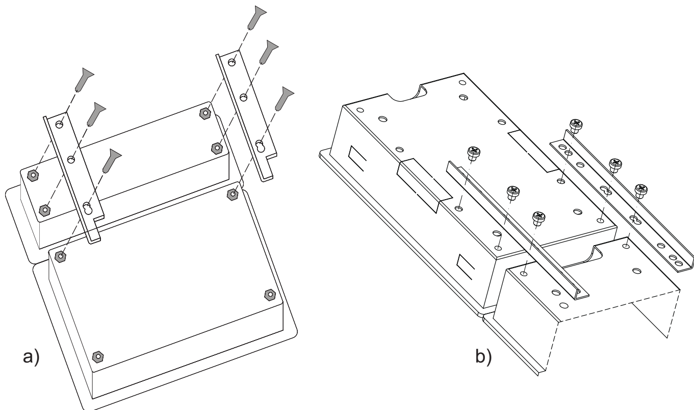
Figure 19: Manner of connecting panel with tenants list with the aid of established elements a) CP-251x and CP-252x panels, b) CP-253x panels
